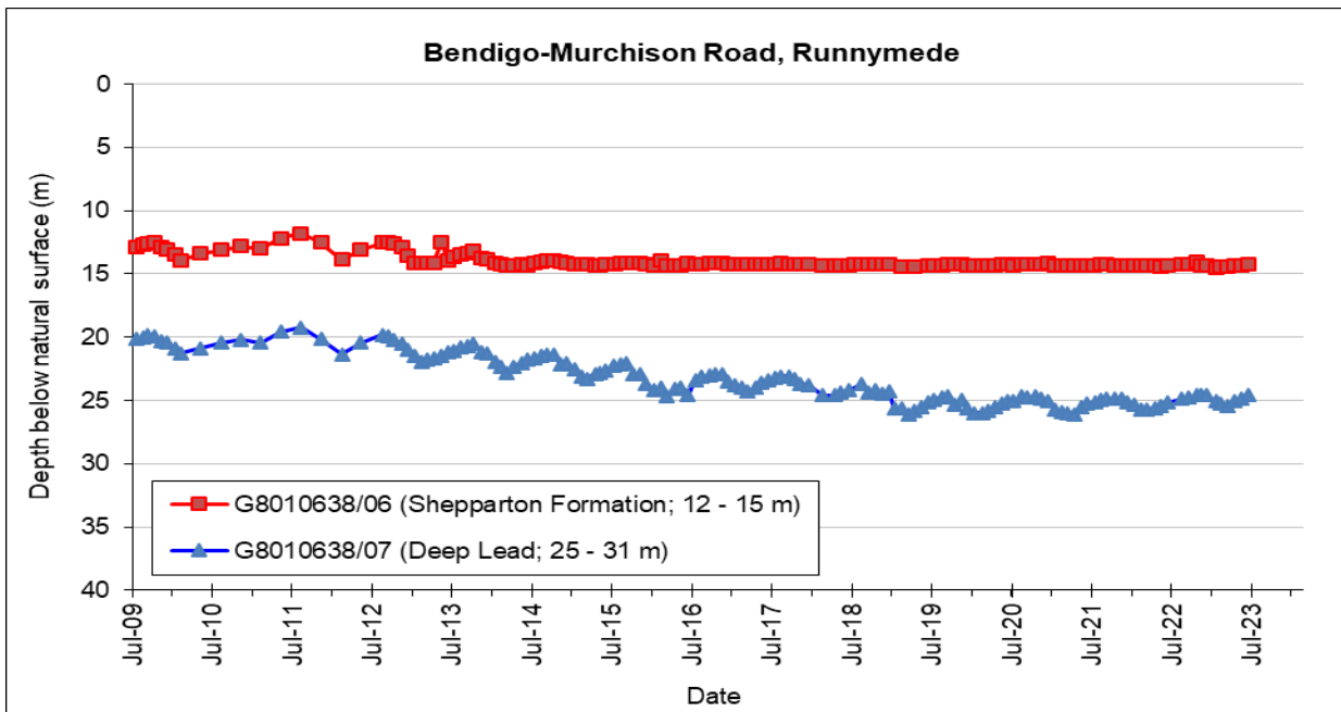
Figure 10 Groundwater level monitoring in the Barnadown Zone, at Runnymede – July 2009 to June 2023 (DELWP, 2023)
