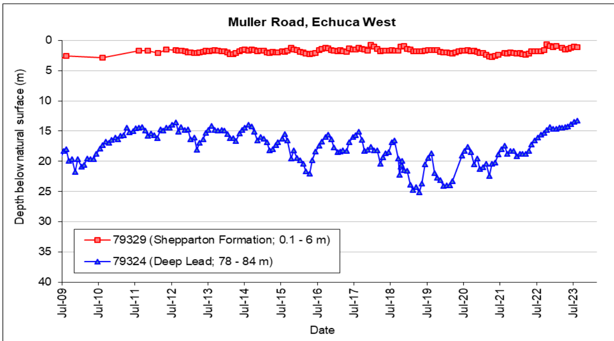
Figure 9 Groundwater level monitoring in the Echuca Zone, at Echuca West – July 2009 to June 2023 (DELWP, 2023)
