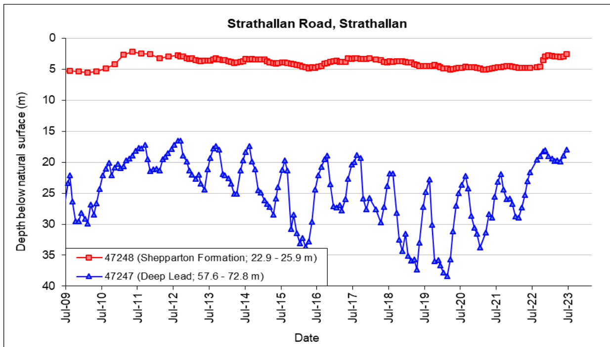
Figure 8 Groundwater level monitoring in the Bamawm Zone, at Strathallan – July 2009 to June 2023 (DELWP, 2023)
